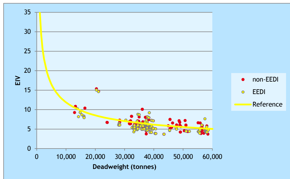
Figure 23 EIV of EEDI and non-EEDI ships (built in 2014-2015): Bulk carriers
